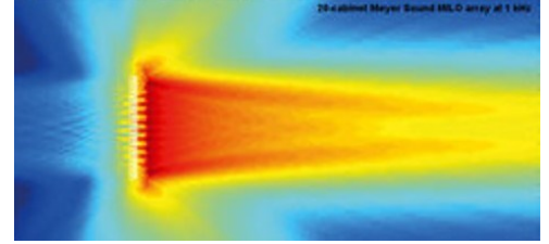
LINE ARRAY
